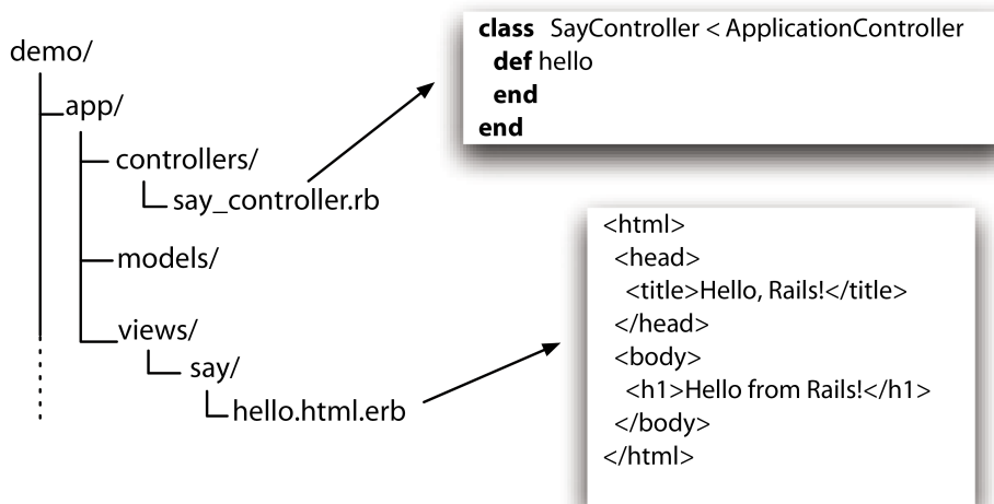
Figure 2—Standard locations for controllers and views
