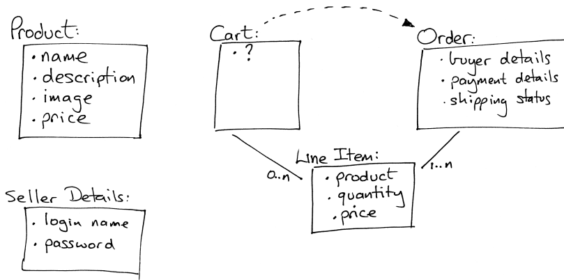
Figure 9—Initial guess at application data
