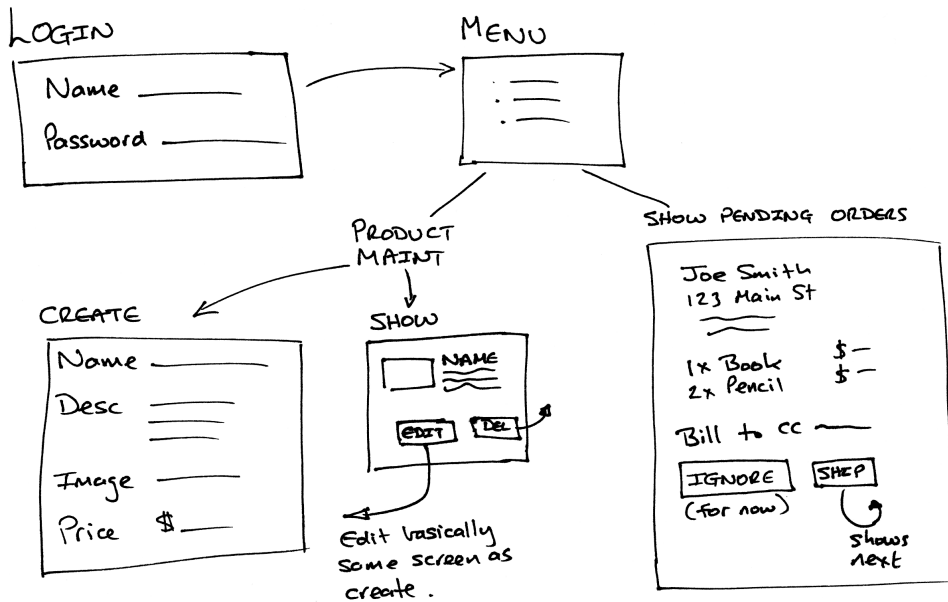
Figure 8—Flow of seller pages
