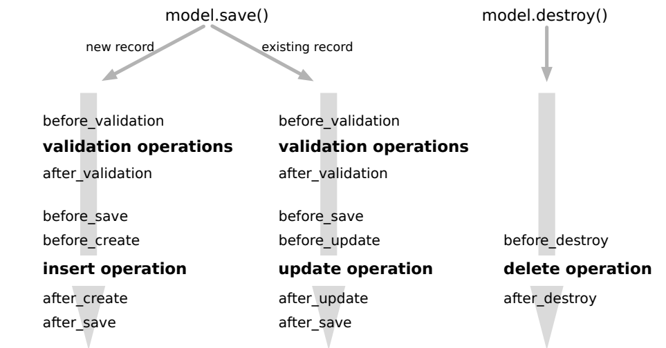
Figure 57—Sequence of Active Record callbacks
