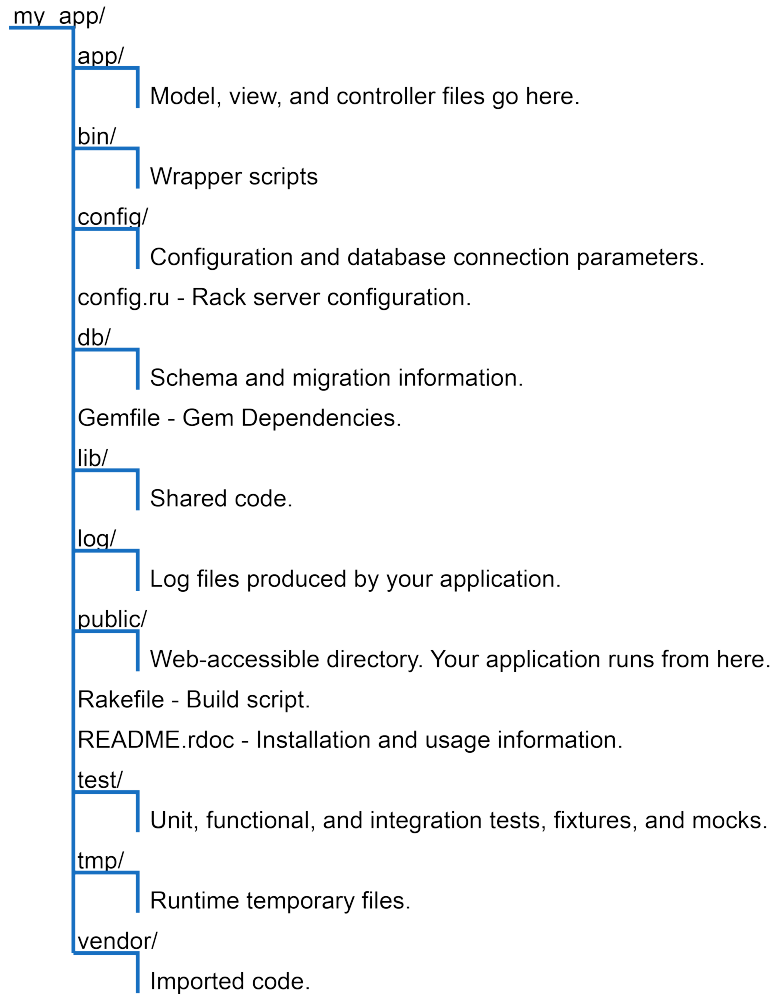
Figure 55—All Rails applications have this top-level directory structure.
