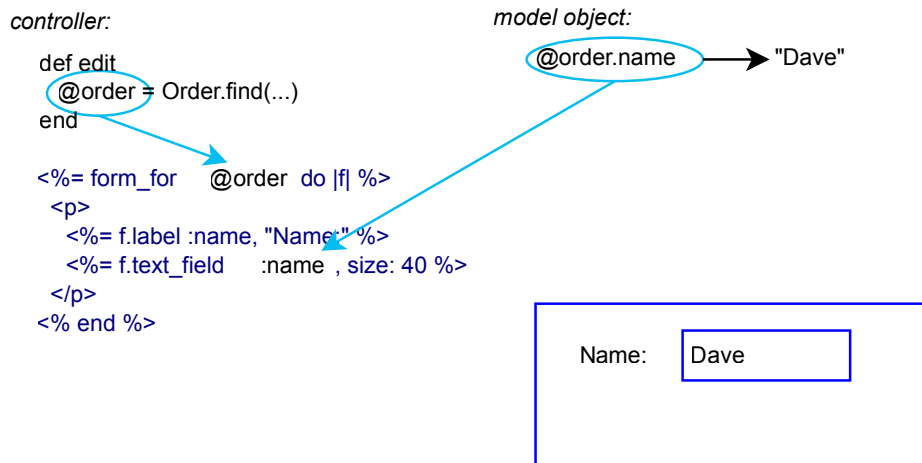
Figure 32—The names in form_for map to objects and attributes.
