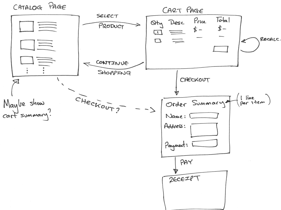
Figure 7—Flow of buyer pages
